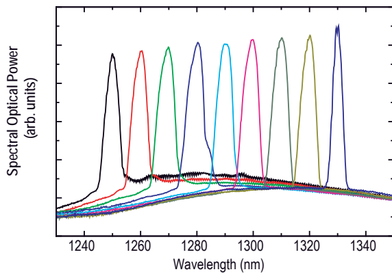
Wavelength Tuning
