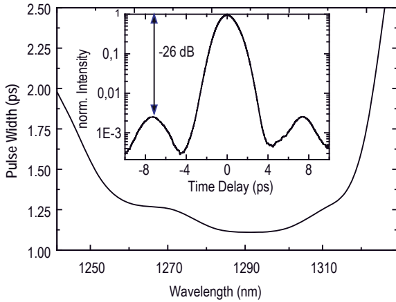
Pulse width an Trailing Pulse Suppression
